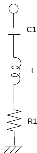
Fig.12 The equivalent circuit using L
