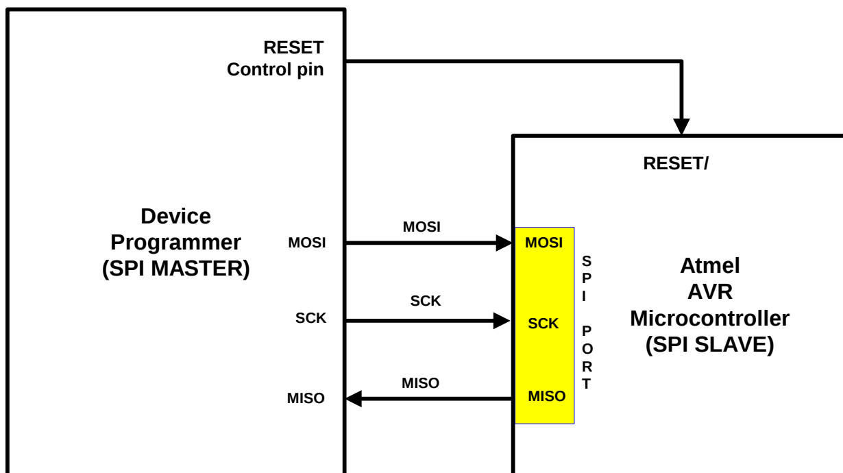
Fig 2.2a – ISP Programming Implementation of Atmel AVR Microcontrollers
