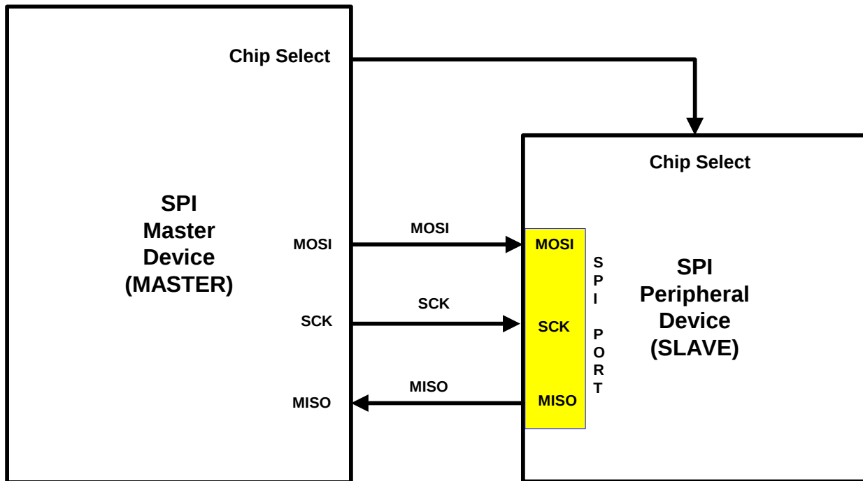
Fig 2.1a – SPI Master / Slave example
