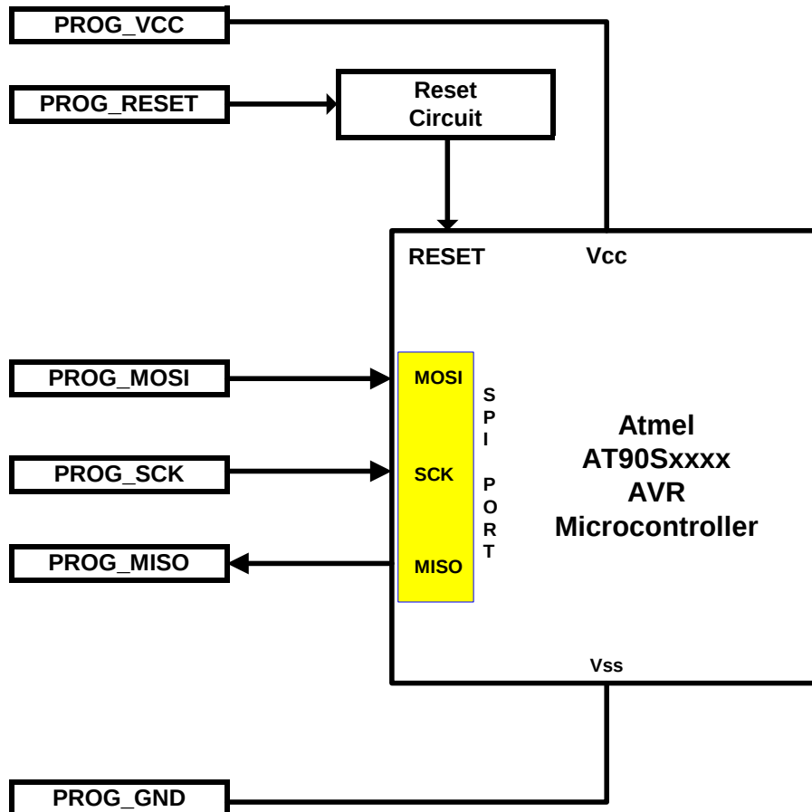
Fig 2.3a AT90Sxxxx AVR – ISP Connections
