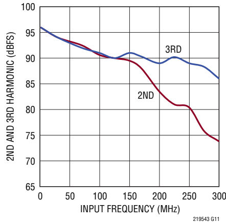
LTC2195: 2nd, 3rd Harmonic vs Input Frequency, -1dBFS, 125Msps, 1V Range
