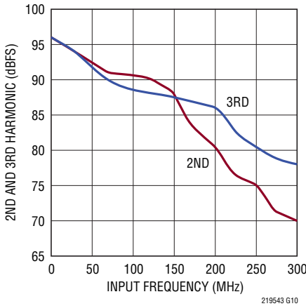
LTC2195: 2nd, 3rd Harmonic vs Input Frequency, -1dBFS, 125Msps, 2V Range
