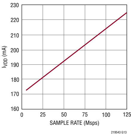
LTC2195: I_{VDD} vs Sample Rate, 5MHz, -1dBFS Sine Wave Input
