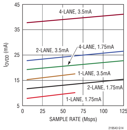
LTC2195: I_{OVDD} vs Sample Rate, 5MHz, -1dBFS Sine Wave Input
