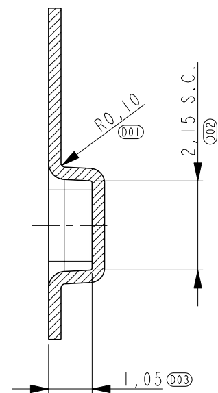
SECTION X - X
