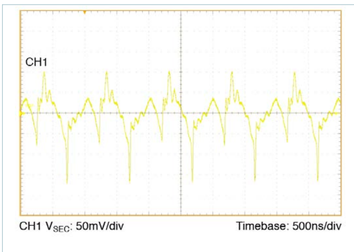
Figure 14 — Full load ripple, 10\mu\text{F } C_{PRI\_IN\_EXT} ; No external C_{SEC\_OUT\_EXT} . Board mounted module, scope setting: 20MHz analog BW
