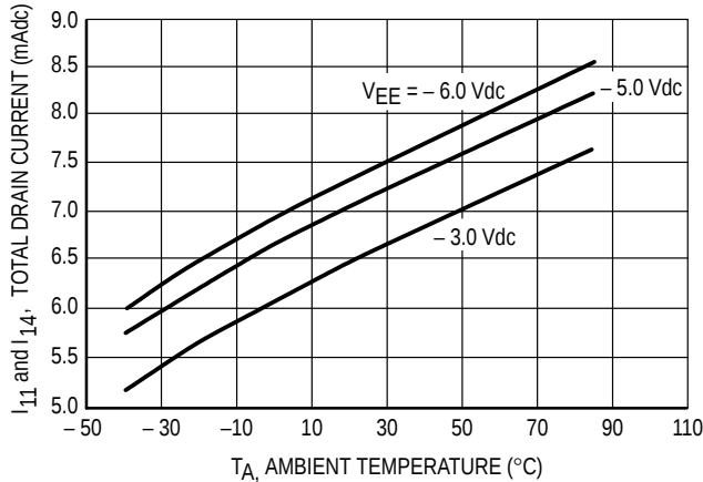
Figure 5. Total Drain Current versus Ambient Temperature and Supply Voltage
