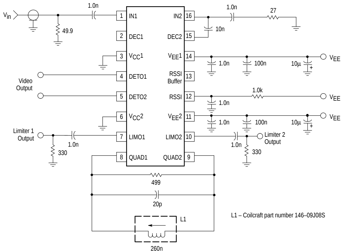
Figure 2. Test Circuit
