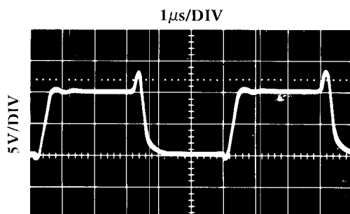
Figure 20. Output Waveform
