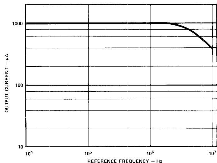
Figure 3. Output Current Bandwidth
