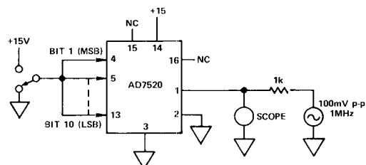
Figure 8. Output Capacitance
