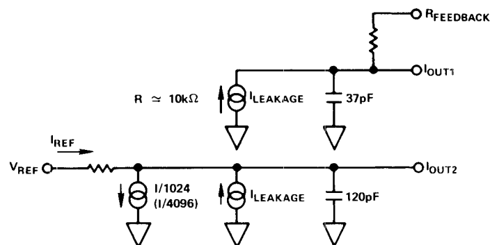
Figure 13. AD7520 (AD7521) Equivalent Circuit—All Digital Inputs Low
