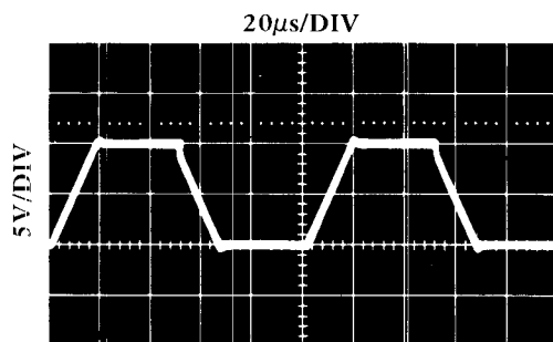
Figure 18. Output Waveform
