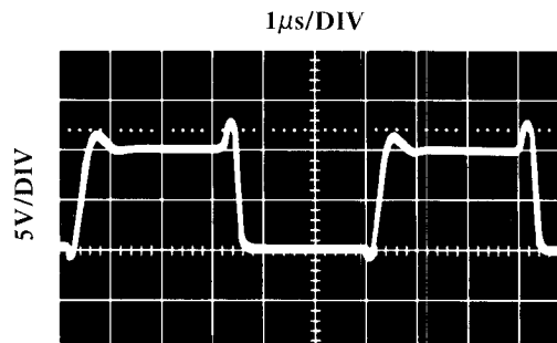
Figure 24. Output Waveform
