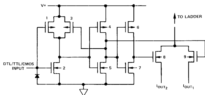
Figure 12. CMOS Switch
