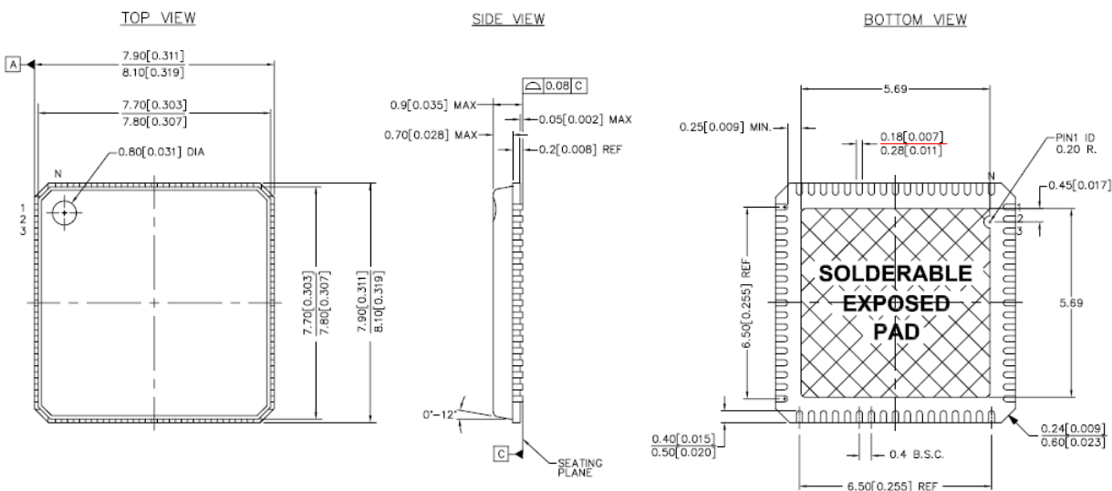
Figure 11-3. 68-Pin (8x8 mm x 0.89 mm) QFN
