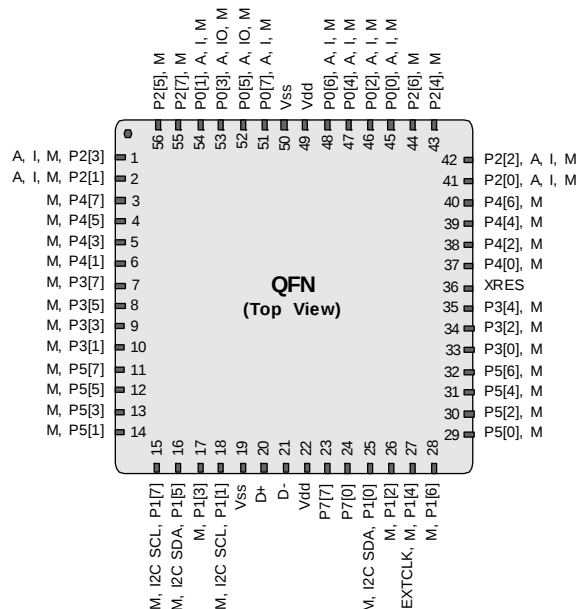
Figure 8-2. CY8C24894 56-Pin PSoC Device
