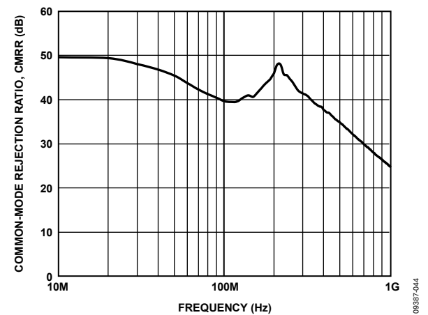
Figure 46. Common-Mode Rejection Ratio vs. Frequency
