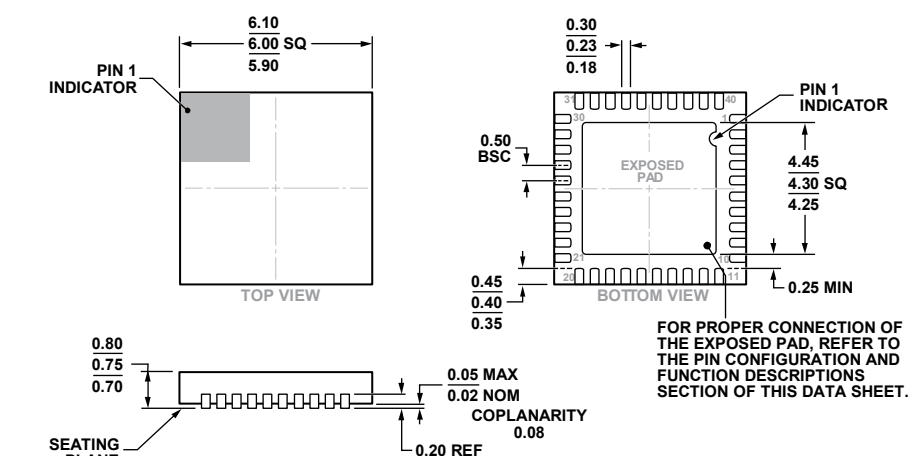
Figure 66. 40-Lead Lead Frame Chip Scale Package [LFCSP_WQ]
