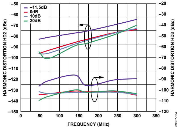
Figure 30. Harmonic Distortion vs. Frequency at Four Gain Codes, Low Power Mode
