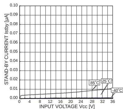
Fig.4 Standby current
