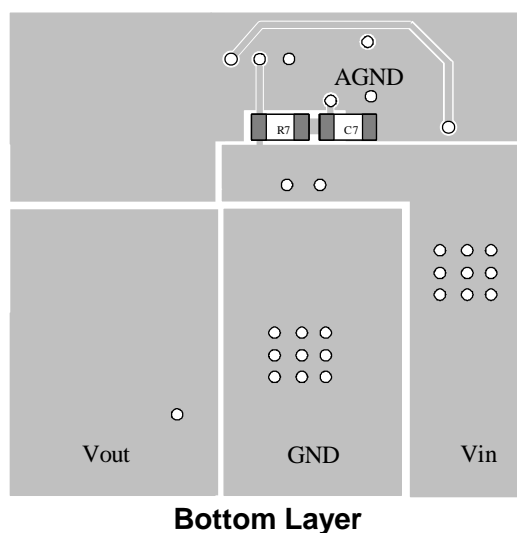
Figure 15—PCB Layout
