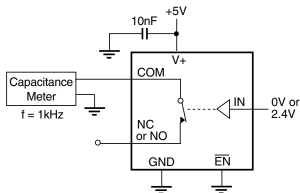
Figure 6. Channel-On Capacitance
