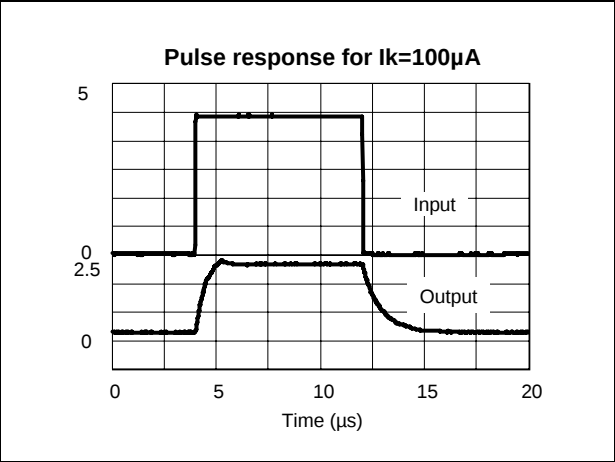
Figure 10. Pulse response for I_k=100\mu A (detailed part)
