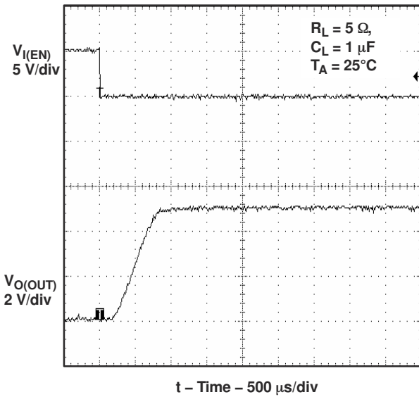
Figure 6-2. Turnon Delay and Rise Time With 1- \mu\text{F} Load
