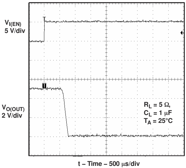
Figure 6-3. Turnoff Delay and Fall Time With 1- \mu\text{F} Load
