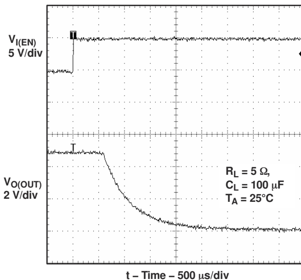
Figure 6-5. Turnoff Delay and Fall Time With 100- \mu F Load
