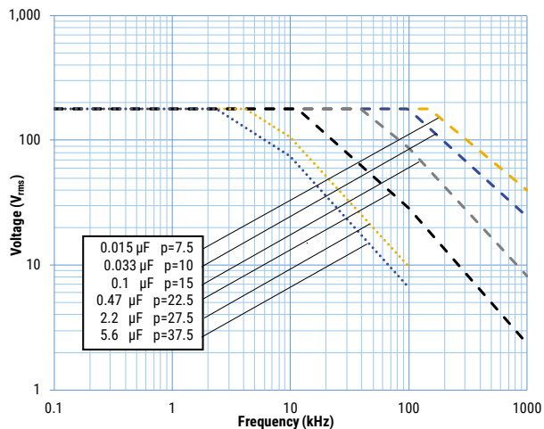
250 VDC/180 VAC
