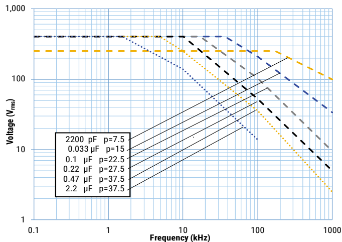
630 VDC/400 VAC
