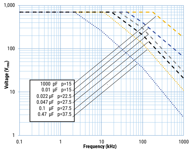
2,000 VDC/700 VAC
