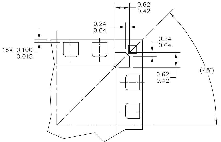
DETAIL M
