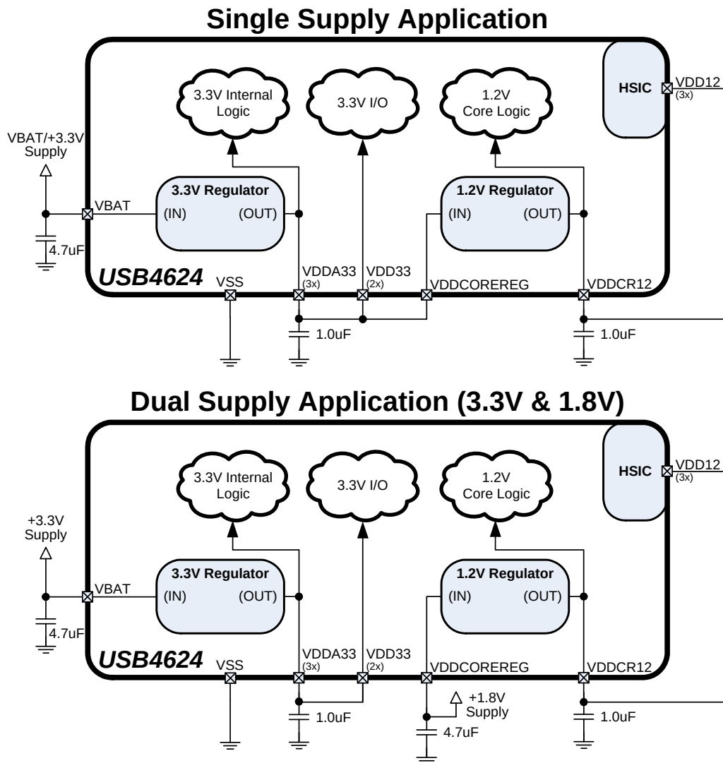
Figure 4.1 Power Connections
