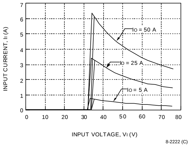
Figure 1. Typical FW250F1 Input Characteristics at Room Temperature
