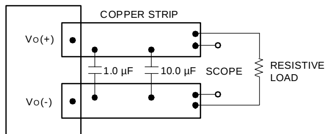
Figure 15. Output Voltage and Efficiency Measurement Test Setup
