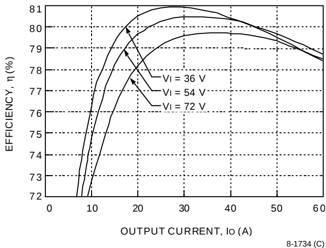
Figure 6. Typical FW300F1 Efficiency vs. Output Current at Room Temperature
