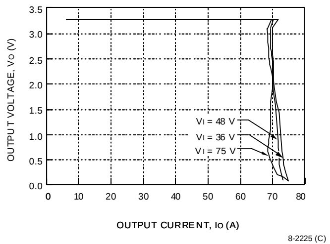
Figure 4. Typical FW300F1 Output Characteristics at Room Temperature
