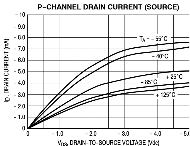
Figure 3. V_{GS} = -5.0 \text{ Vdc}
