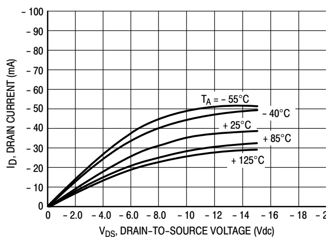
Figure 7. V_{GS} = -15 \text{ Vdc}
