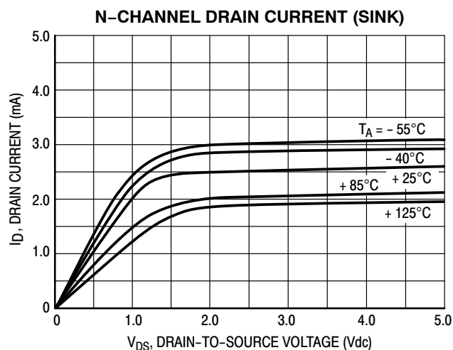
Figure 2. V_{GS} = 5.0 \text{ Vdc}
