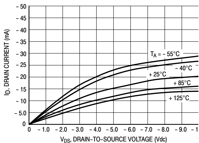
Figure 5. V_{GS} = -10 \text{ Vdc}
