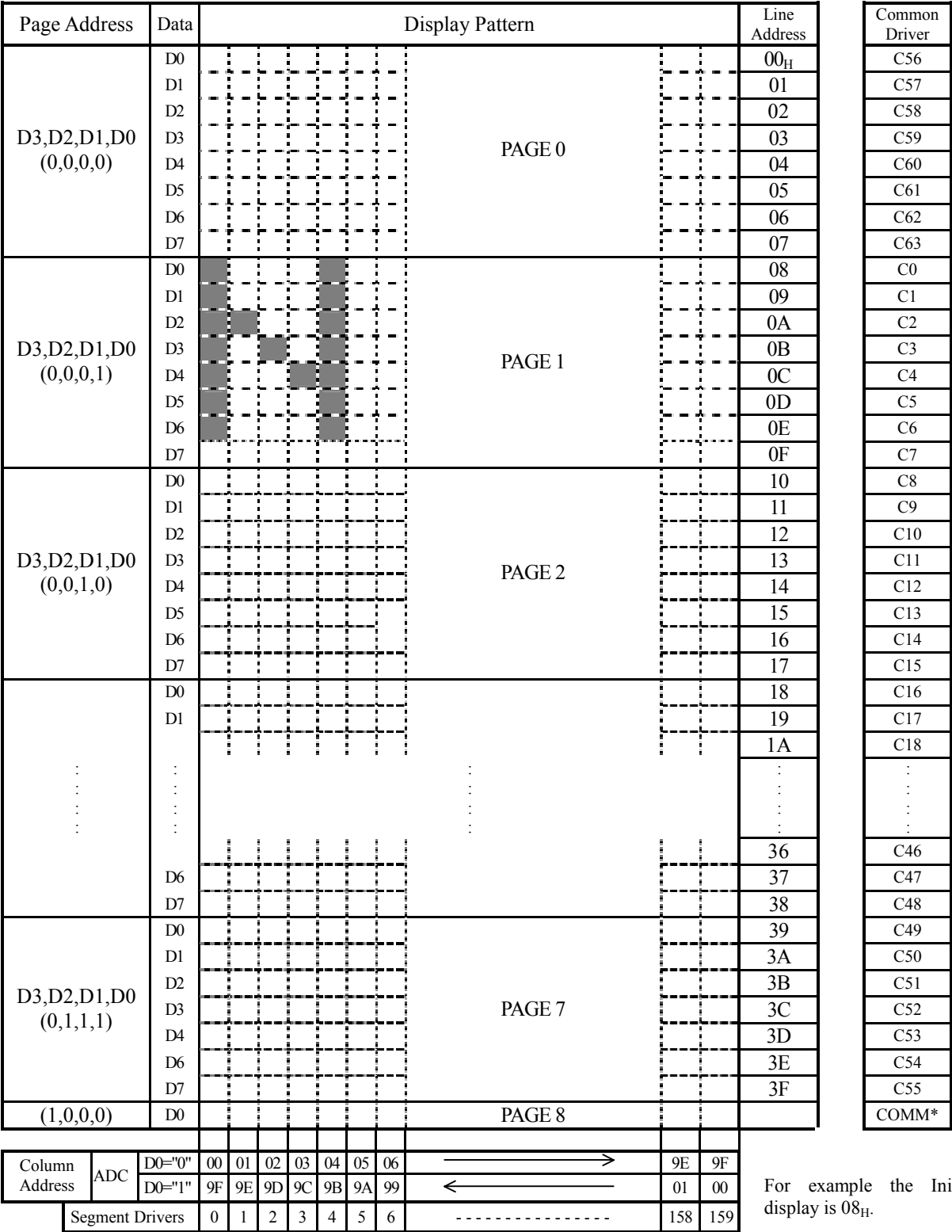
Fig.1 Display data RAM (DDRAM) Map
