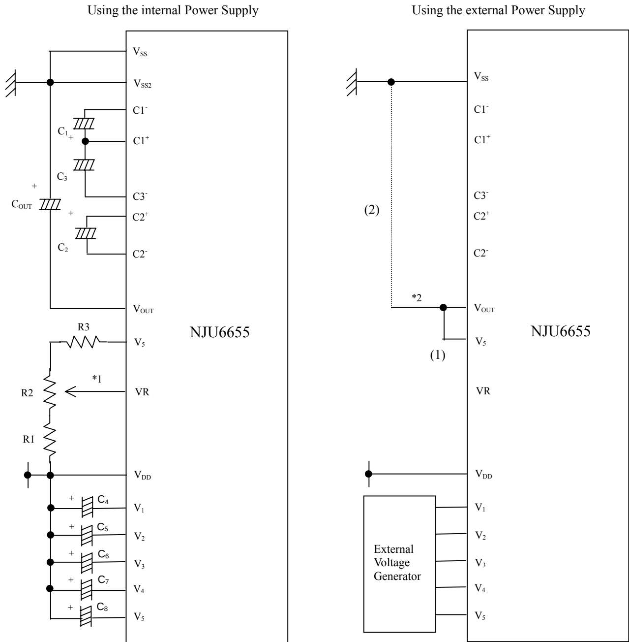
Fig.4 LCD Driving Voltage Generation Circuits
