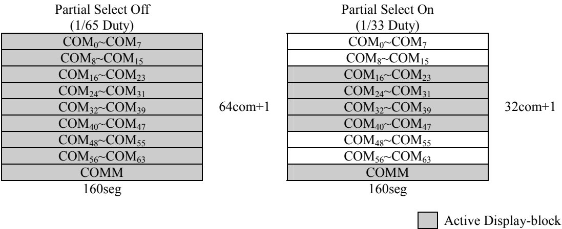
Display structure by Partial Select On / Off
