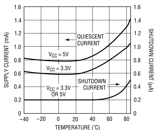
Supply Current
