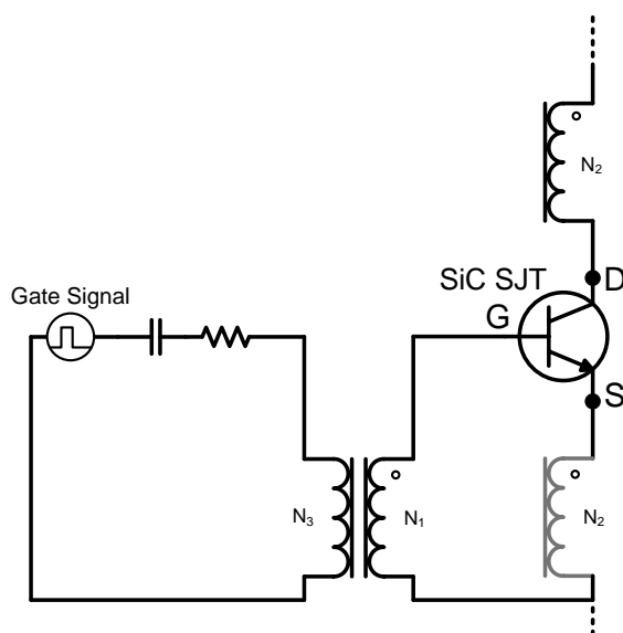
Figure 28: Simplified Current Controlled Proportional Driver
