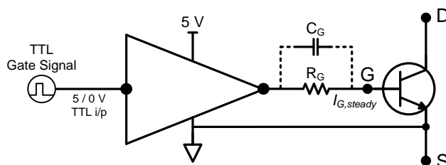
Figure 21: TTL Gate Drive Schematic
