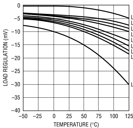
Load Regulation \Delta I_L = 1\text{mA} to 50mA
