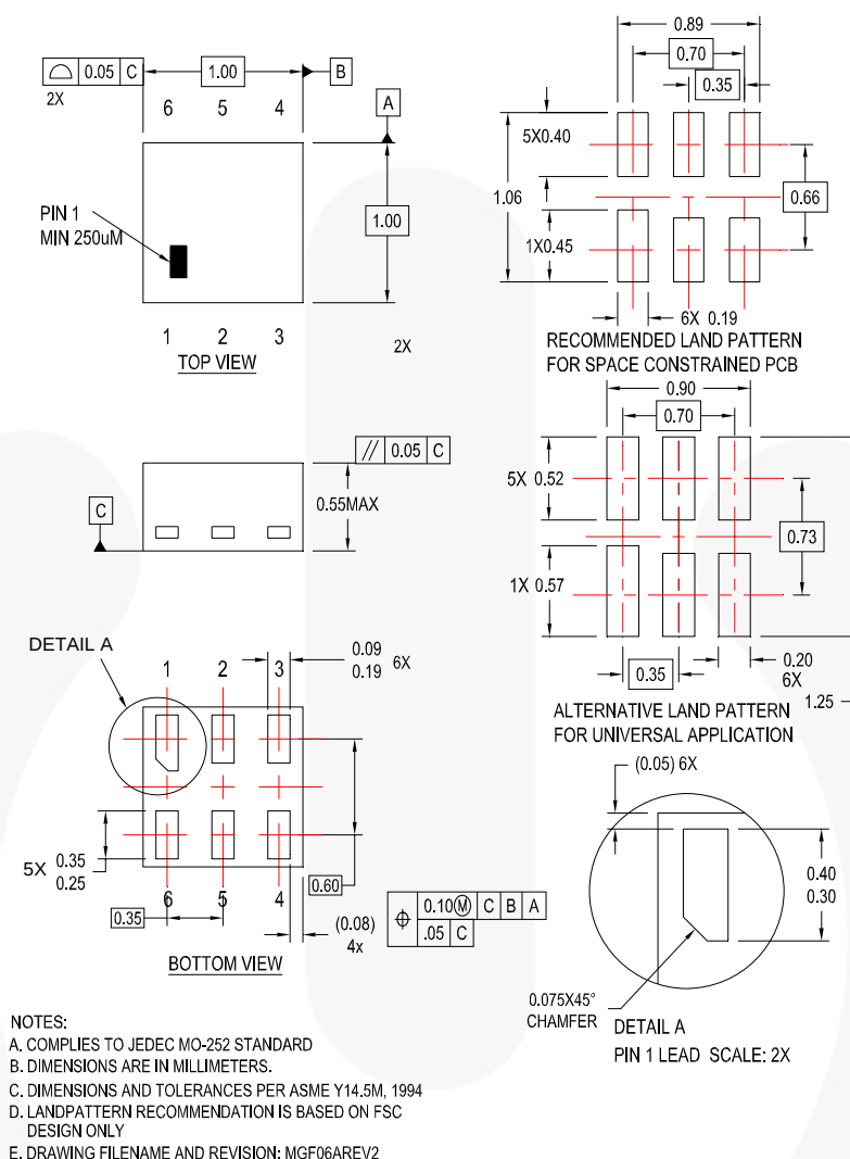
Figure 19. 6-Lead, MicroPak2, 1x1mm Body, .35mm Pitch
