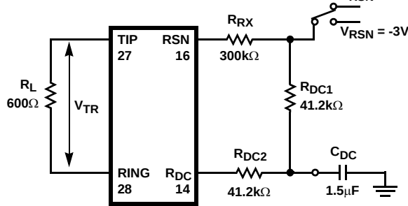
FIGURE 8. CURRENT GAIN-RSN TO METALLIC
