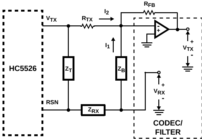
FIGURE 17. TRANSHYBRID CIRCUIT
