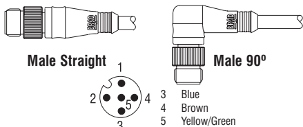
WIRING CONFIGURATION
