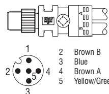
WIRING CONFIGURATION
