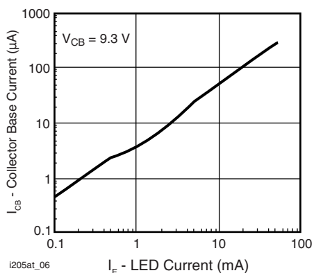
Fig. 7 - Collector Base Photocurrent vs. LED Current
