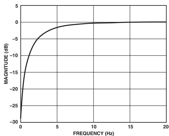
TPC 4. ADC High-Pass Filter Response, f_s = 96 kHz
