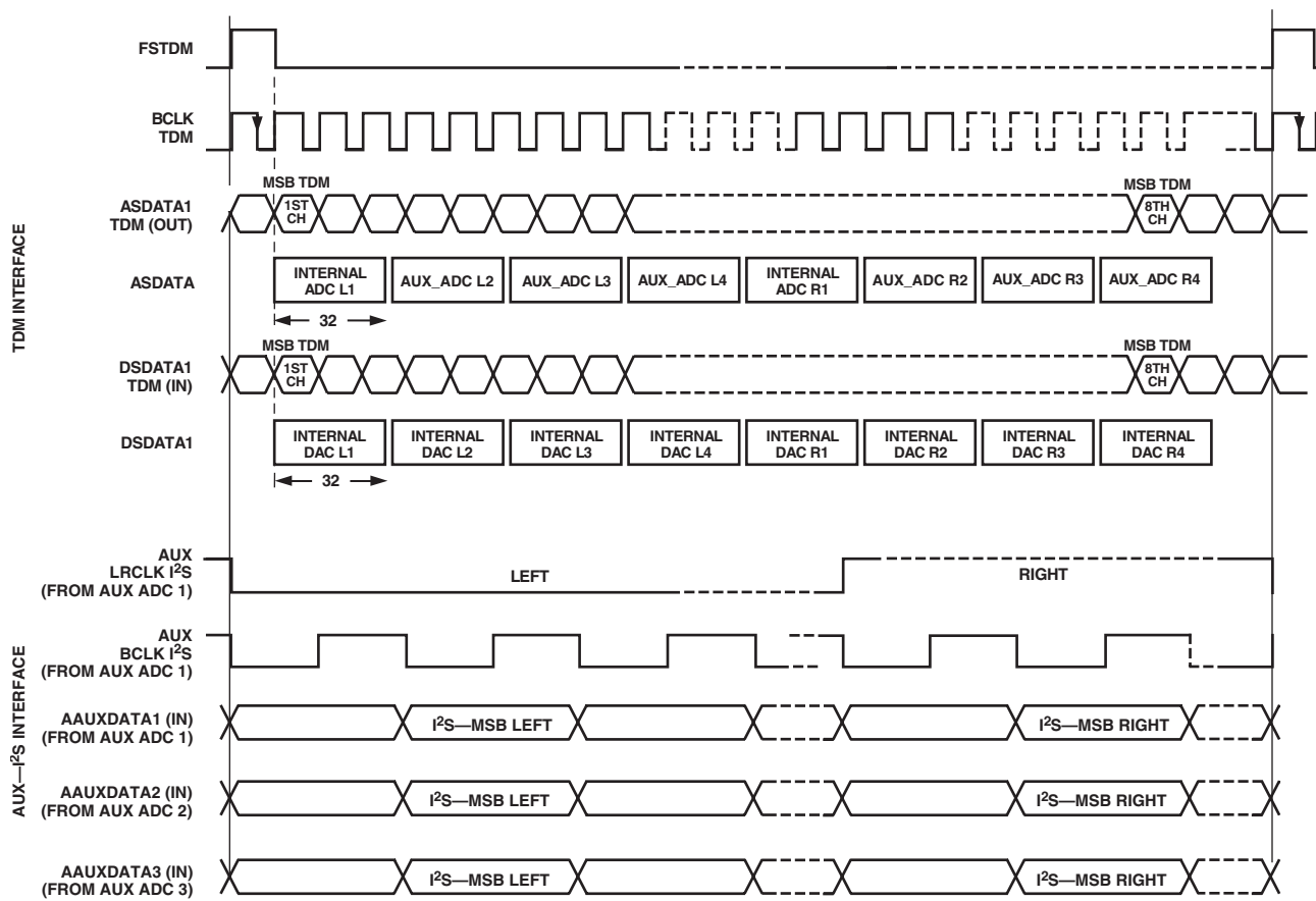
Figure 11. Aux Mode Timing
