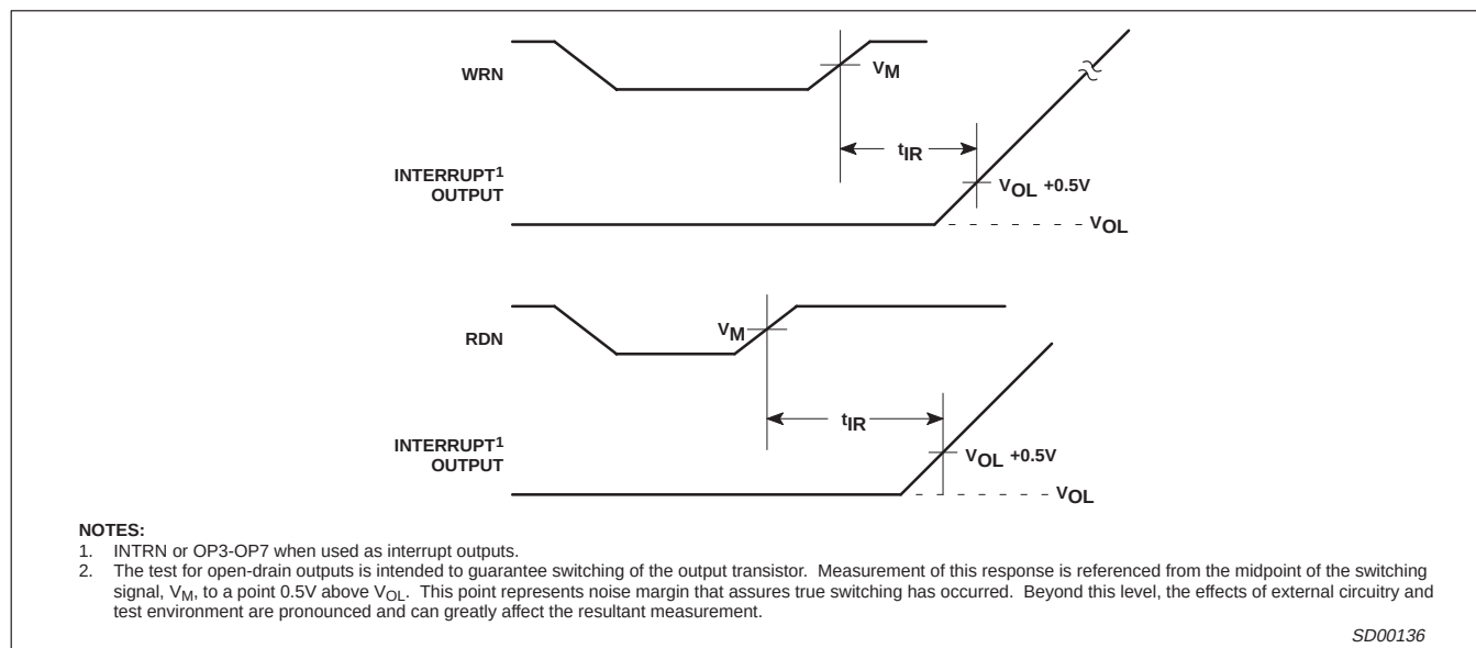
Figure 6. Interrupt Timing
