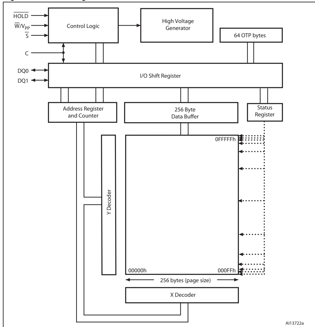
Figure 6. Block diagram
