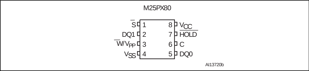
Figure 2. VFQFPN, SO8, and PDIP8 connections
