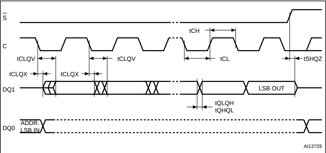
Figure 32. Output timing
