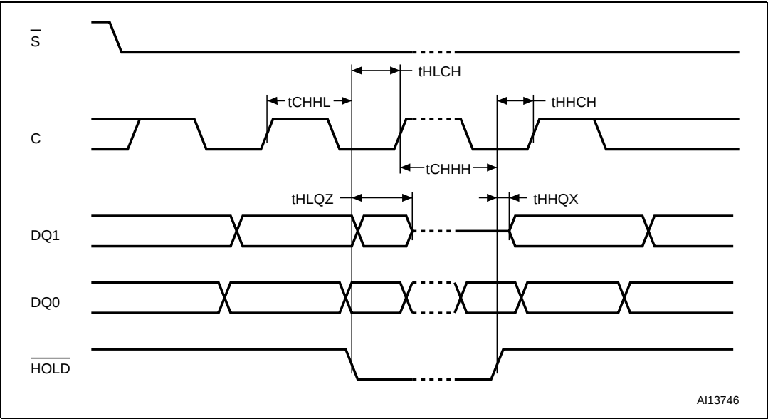
Figure 31. Hold timing
