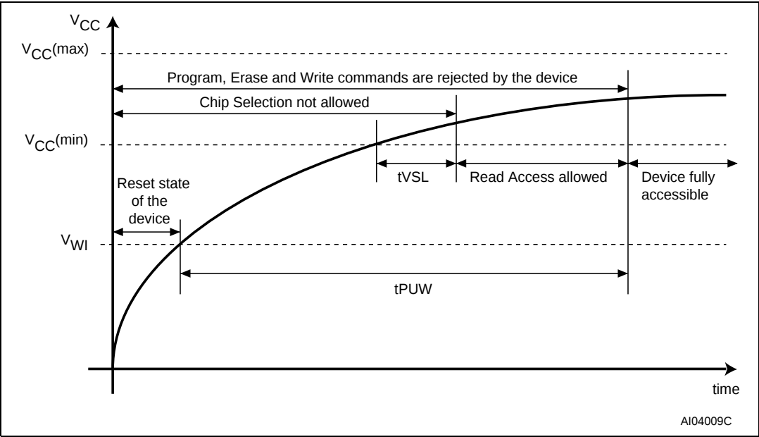
Figure 27. Power-up timing
