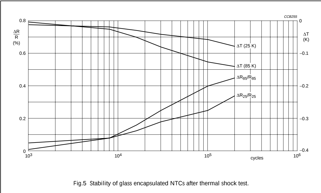
Stability and R-T characteristics
