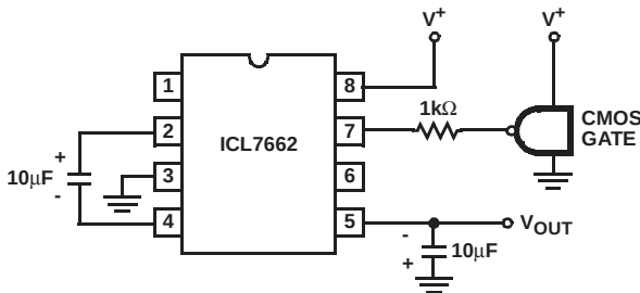
FIGURE 20. EXTERNAL CLOCKING
