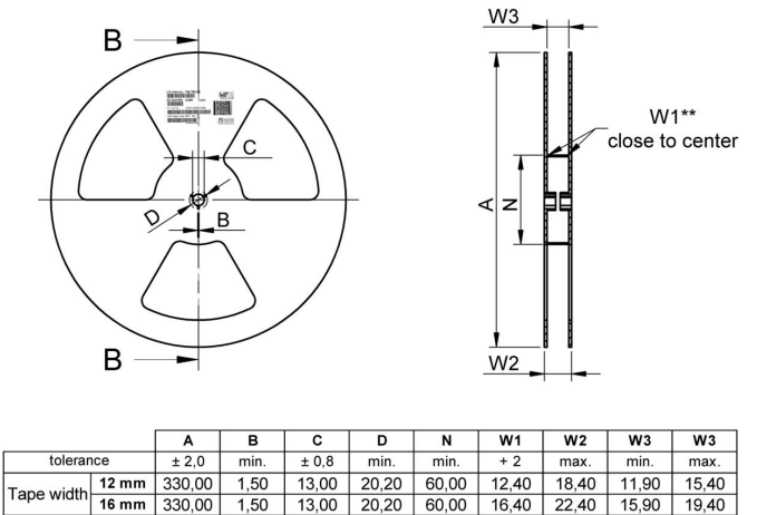
sectional drawing B-B
