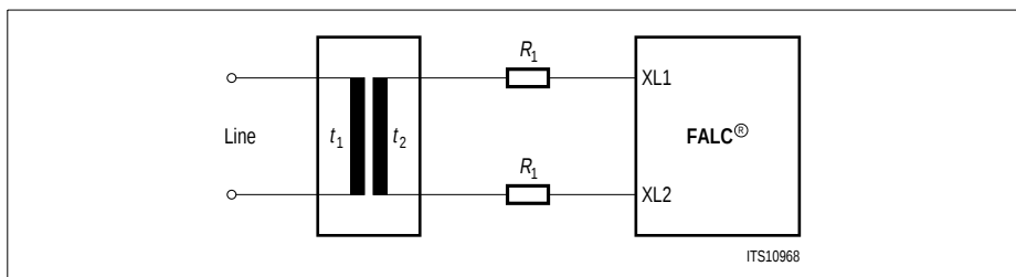
Figure 23 Transmitter Configuration (E1)
