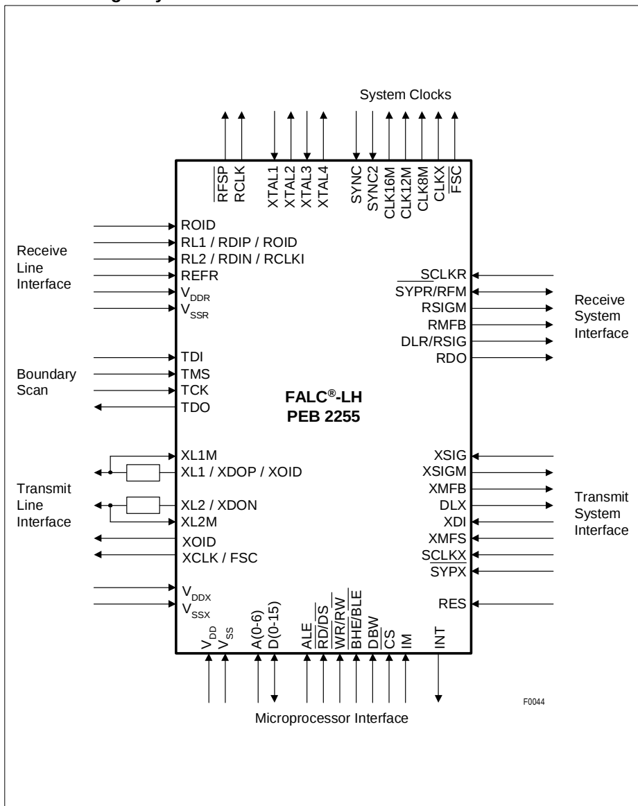
Figure 1 Logic Symbol
