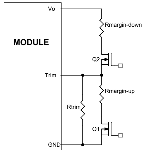
Circuit Configuration for margining Output voltage
