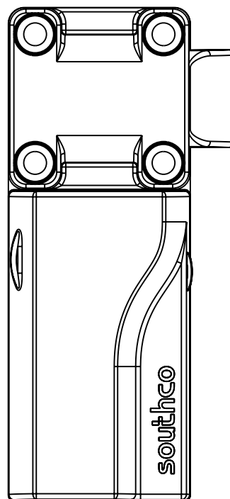
LATCH BOLT RIGHT ORIENTATION EM-10-12-XXX-X
