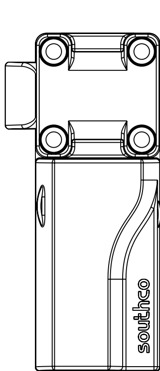
LATCH BOLT LEFT ORIENTATION EM-10-13-XXX-X
