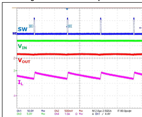
Figure 17. Short-circuit protection
