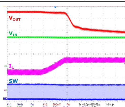
Figure 16. Overcurrent protection
