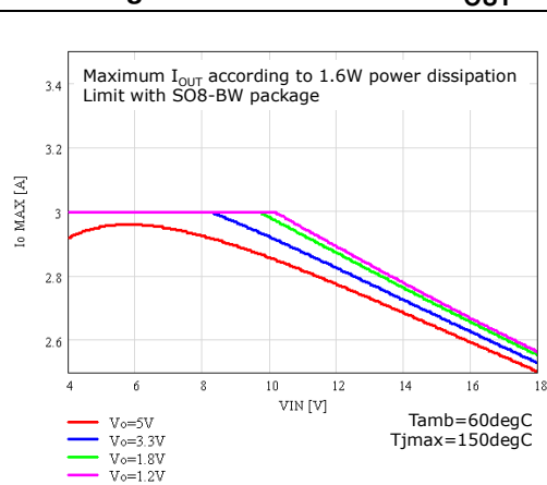
Figure 18. SO8 maximum I_{OUT}
