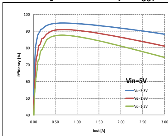
Figure 13. Efficiency vs. I_{OUT}
