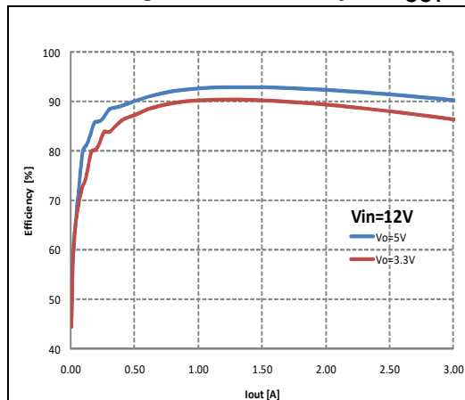
Figure 15. Efficiency vs. I_{OUT}
