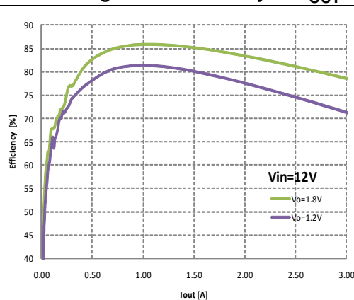
Figure 14. Efficiency vs. I_{OUT}
