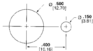
Recommended Panel Cut-out Shielded with Front Panel Screw-Down
