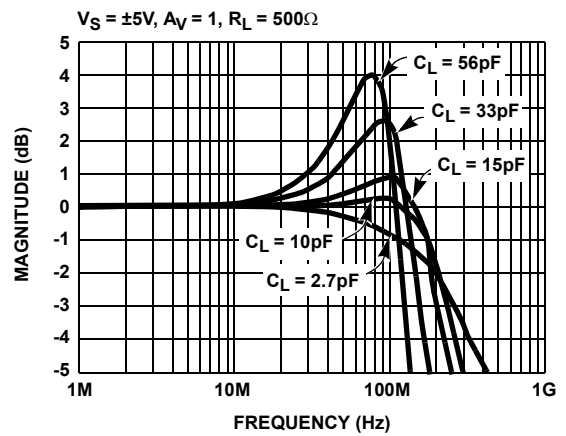
FIGURE 4. FREQUENCY RESPONSE vs C_L
