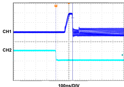
FIGURE 19. ENABLED RESPONSE
