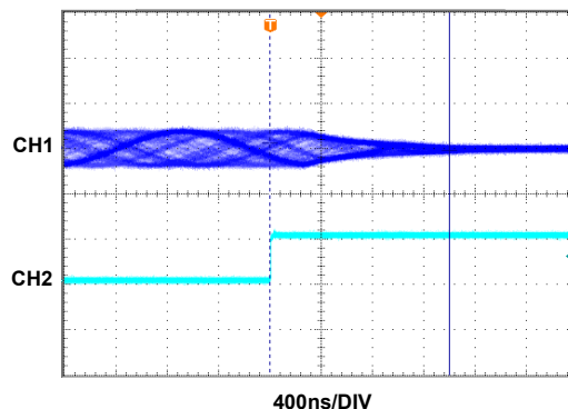
FIGURE 20. DISABLED RESPONSE
