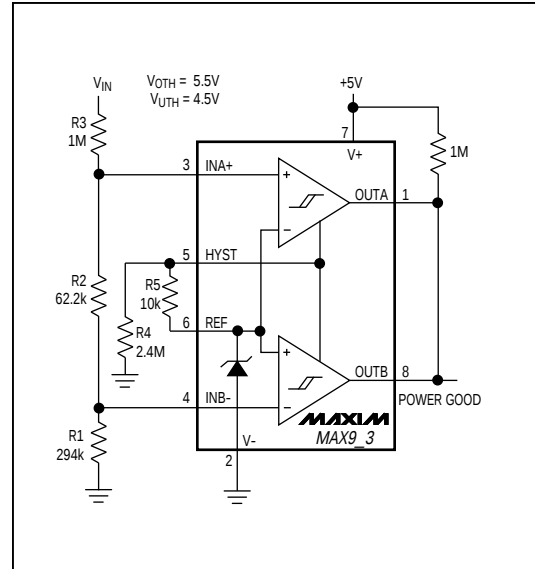
Figure 5. Window Detector
