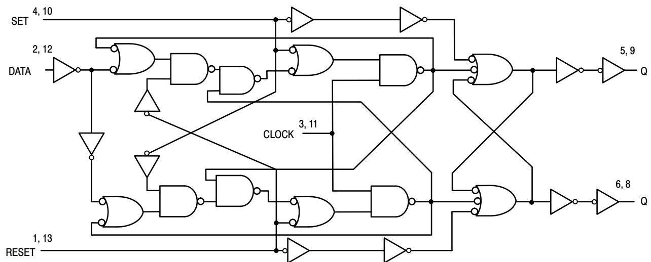
Figure 7. Expanded Logic Diagram
