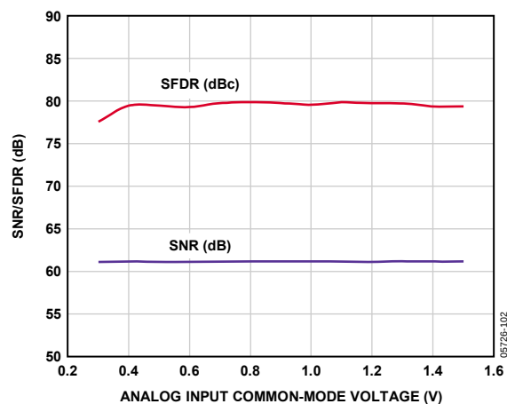
Figure 46. SNR/SFDR vs. Common-Mode Voltage, f_{IN} = 2.4 MHz, f_{SAMPLE} = 40 MSPS
