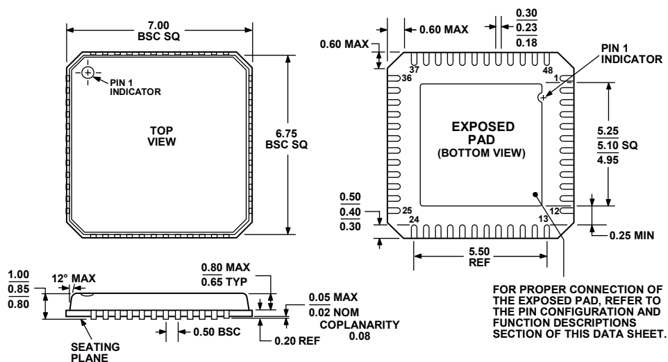
Figure 82. 48-Lead Lead Frame Chip Scale Package [LFCSP_VQ] 7 mm × 7 mm Body, Very Thin Quad (CP-48-1)
