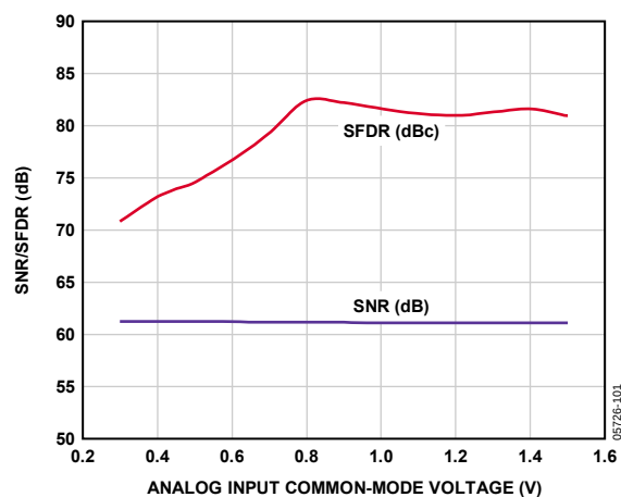
Figure 47. SNR/SFDR vs. Common-Mode Voltage, f_{IN} = 30 MHz, f_{SAMPLE} = 40 MSPS
