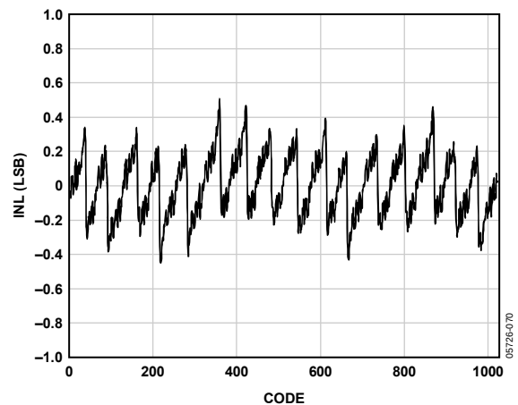
Figure 37. INL, f_{IN} = 2.4 MHz, f_{SAMPLE} = 65 MSPS
