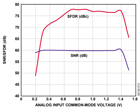
Figure 45. SNR/SFDR vs. Common-Mode Voltage, f_{IN} = 30 MHz, f_{SAMPLE} = 65 MSPS
