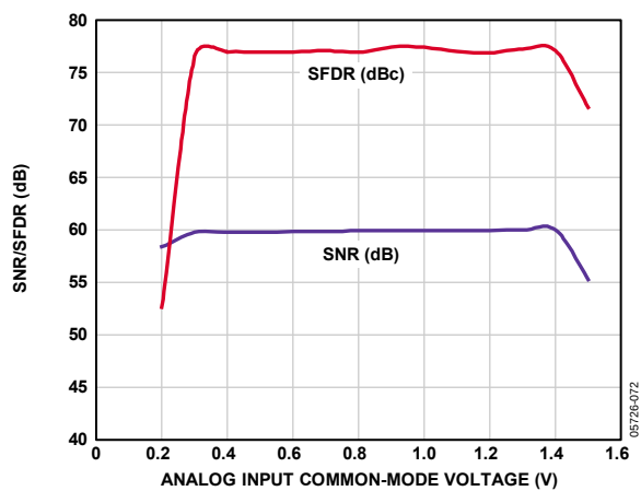
Figure 44. SNR/SFDR vs. Common-Mode Voltage, f_{IN} = 2.4 MHz, f_{SAMPLE} = 65 MSPS
