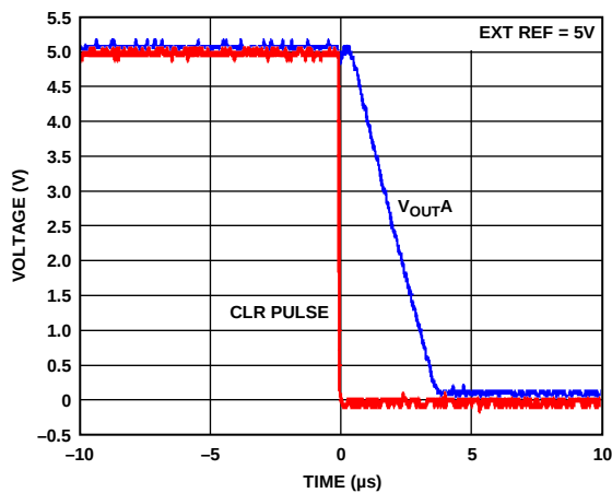
Figure 44. Hardware \overline{CLR}
