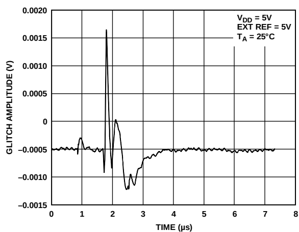
Figure 37. DAC-to-DAC Crosstalk
