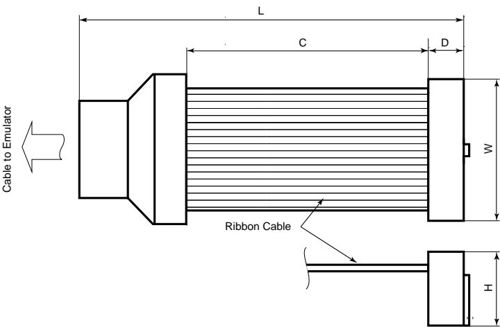
FIGURE 10 Top and side views of the 20-pin ARM probe with a cable extender. L = 69 mm (2.7 in.), C = 40.0 mm (1.55 in.) D = 6.0 mm (.24), W = 30.0 mm (1.2 in.), H = 11.5 mm (0.45 in.).
