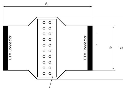
FIGURE 37 The dimensions of the JTAG-ETM splitter board. A = 52.0 mm (2.05 in), B = 25.4 mm (1 in), C = 33.9 mm (1.34 in).
