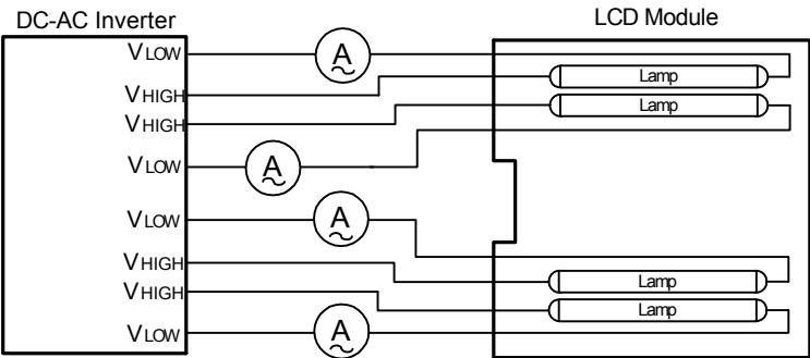
LCD module connection diagram (reference)
