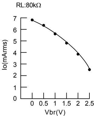
Vbr vs Output Current (reference)
