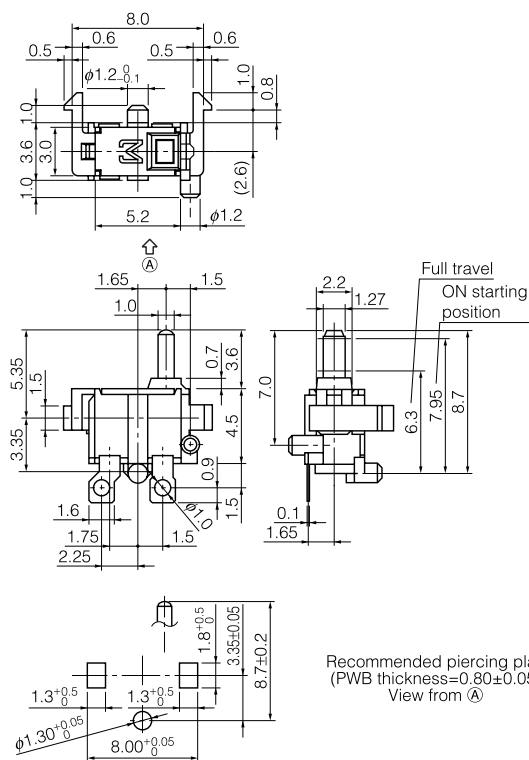
No. 10 ESE11SF3 Snap-in type 1-pole 1-throw
