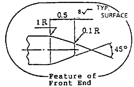
Fig. 1 Gage for Measuring Contact Insertion/Extraction Force
