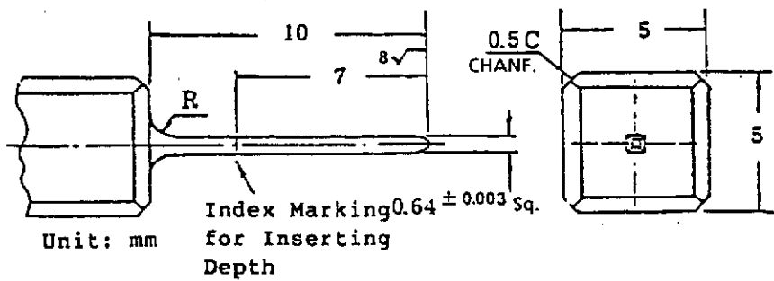
Fig. 1 Gage for Measuring Contact Insertion/Extraction Force
