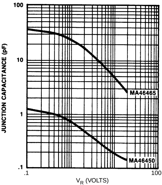
JUNCTION CAPACITANCE vs REVERSE BIAS VOLTAGE ( \gamma = 1.0 ) (CHIPS)
