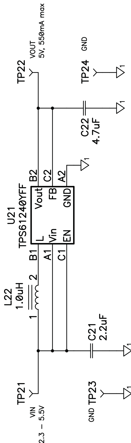
Figure 5. TPS61240EV-360 Schematic – U21 Configuration
