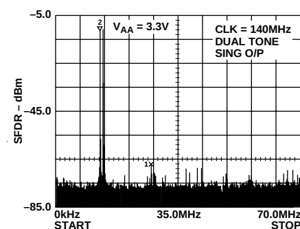
Figure 19. Dual-Tone SFDR @ f_{CLOCK} = 140\text{ MHz} ( f_{OUT1} = 13.5\text{ MHz} , f_{OUT2} = 14.5\text{ MHz} )
